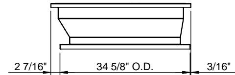
RIGHT VIEW
