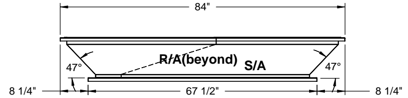
RIGHT VIEW
