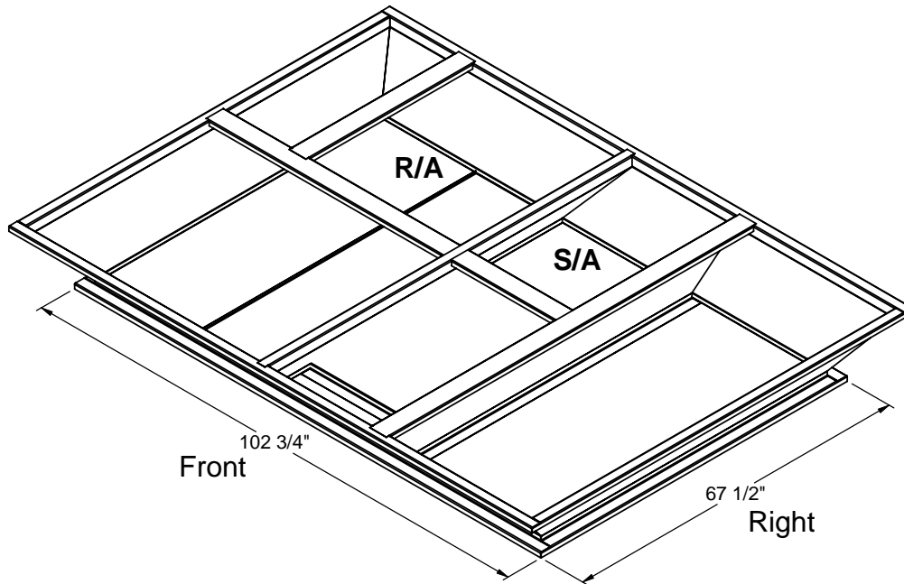
ISOMETRIC VIEW
