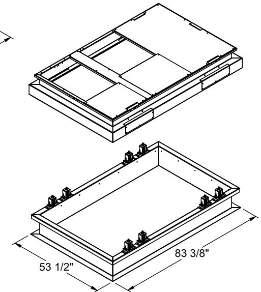
EXPLODED DETAIL
