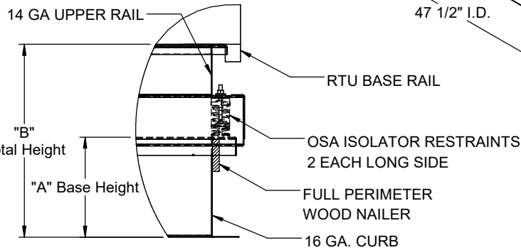
PROFILE DETAIL
