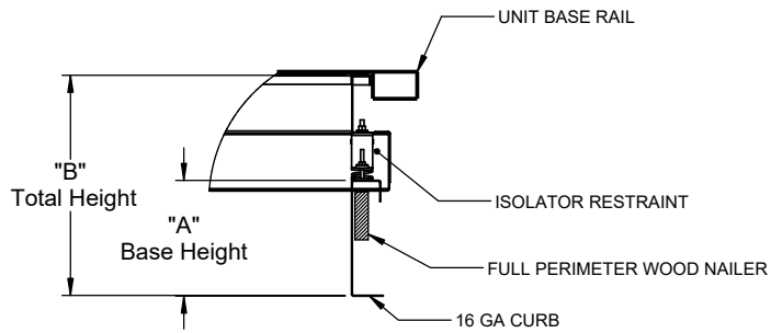
SIDE VIEW DETAIL
