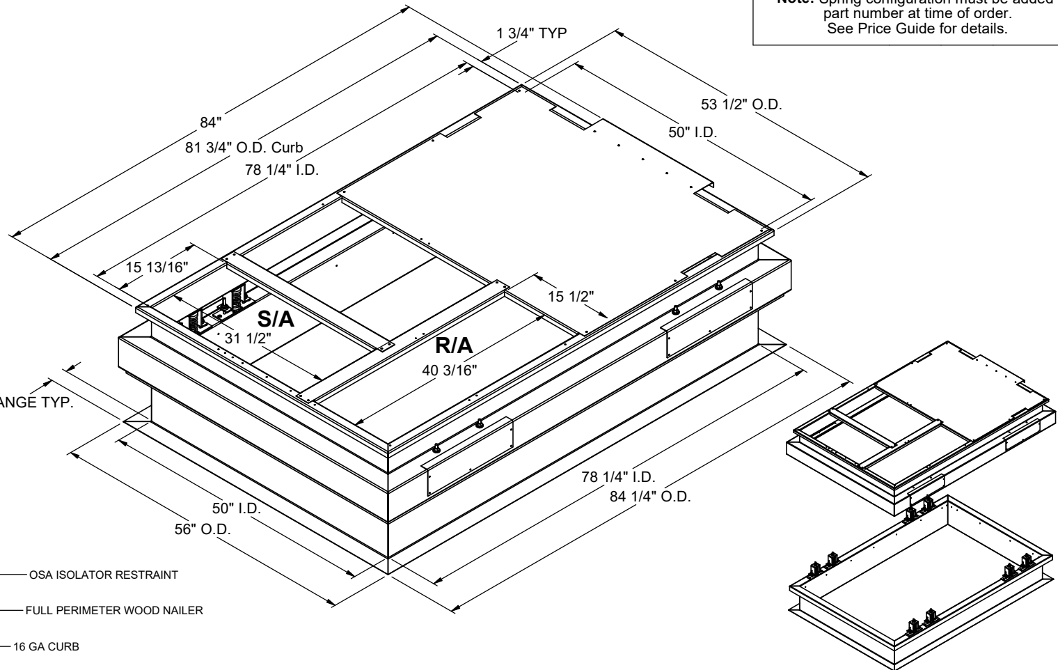
EXPLODED DETAIL
