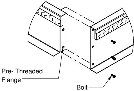
CORNER DETAIL
