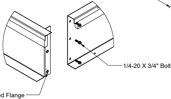
CORNER DETAIL
