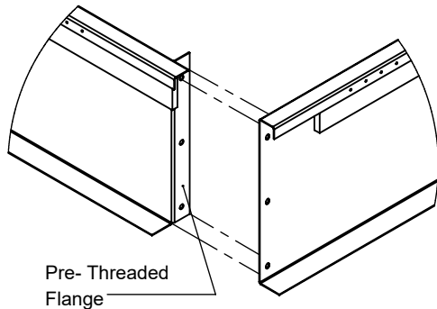
CORNER DETAIL
