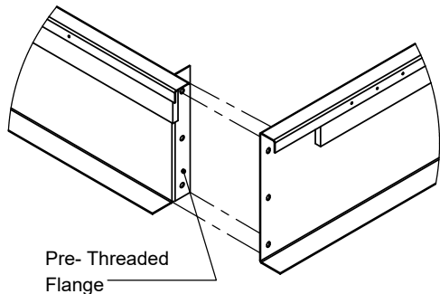
CORNER DETAIL
