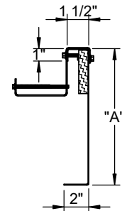
CROSS SECTION DETAIL
