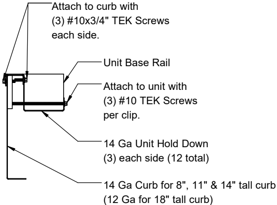
HOLD DOWN DETAIL
