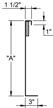
CURB DETAIL
