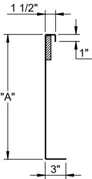
CURB DETAIL
