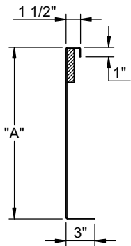
CURB DETAIL
