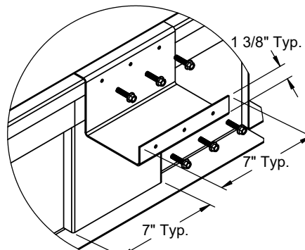
DETAIL K
