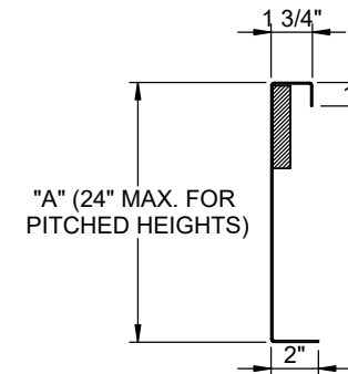
CURB DETAIL
